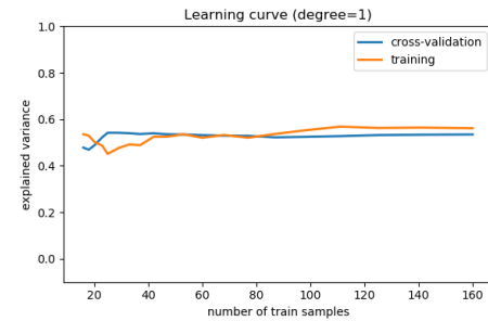
Fig. 5: For a degree=1 model
