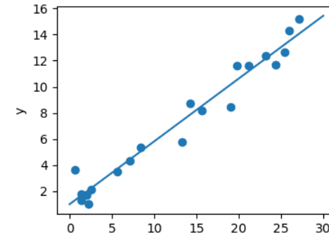
Fig. 4: A plot of a simple linear regression.
