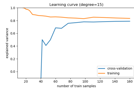
Fig. 6: For a degree=15 model
